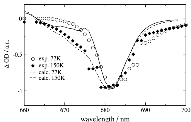
FIGURE 7 Experiments (19) and calculations of the temperature dependence of T-S spectra of Synechocystis sp. PCC 6803. The site energy of \text{Chl}_{\text{D1}} was assumed to change with temperature, corresponding to wavelengths of 680 nm at 77 K and 678 nm at 150 K.
