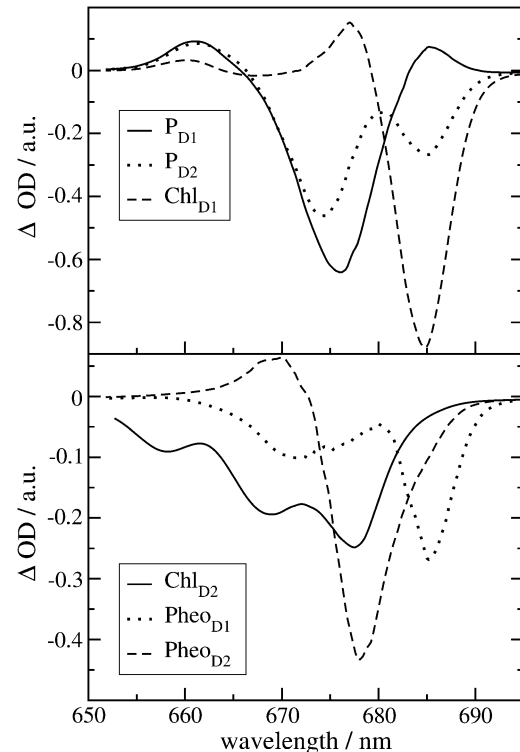
FIGURE 3 T-S spectra at 5 K calculated assuming the triplet state to be localized on the respective reaction center pigments, as indicated in the legends.
