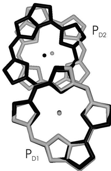
FIGURE 11 Overlay of the special pair (bacterio-) chlorophylls of PS-II (shaded) and the bacterial reaction center (solid). The overlay was determined from a minimization of the mean-square deviation in positions of equivalent atoms of the two molecules using the same program as in Fig. 10.
