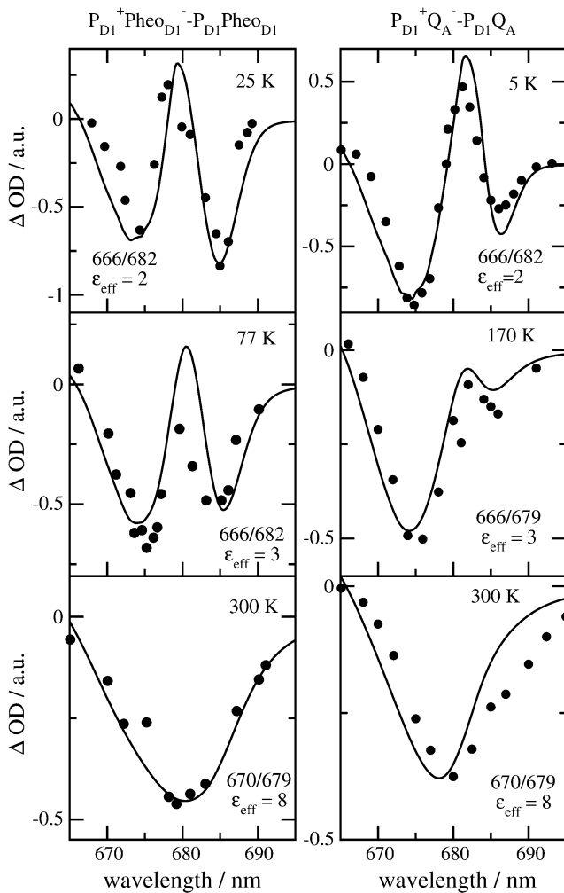
FIGURE 8 Temperature dependence of the P_{D1}^+ \text{Pheo}_{D1}^- - P_{D1} \text{Pheo}_{D1} (left half) and the P_{D1}^+ Q_A^- - P_{D1} Q_A (right half) spectra of T. elongatus . The calculations (solid lines) are compared with experimental data (solid circles) (21). The temperature-dependent wavelengths corresponding to the site energies of P_{D1} and \text{Chl}_{D1} ( P_{D1}/\text{Chl}_{D1} ) and the dielectric constants ( \epsilon_{\text{eff}} ) are shown as well at each temperature.
