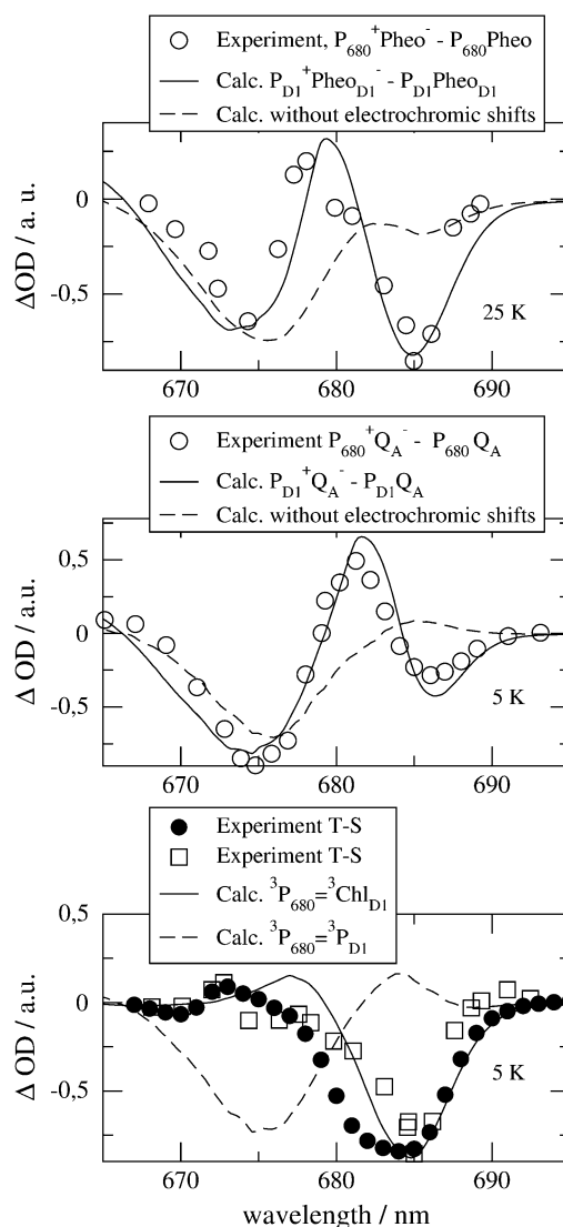
FIGURE 1 Experiments (21) and calculations of optical difference spectra of PS-II core complexes from Thermosynechococcus elongatus . The calculations were performed using the site energies determined previously (18), except for \text{Chl}_{D1} which was shifted by 4 nm to the red. The corresponding wavelengths assigned to each pigment are P_{D1} , 666 nm; P_{D2} , 666 nm; \text{Chl}_{D1} , 682 nm; \text{Chl}_{D2} , 667 nm; \text{Pheo}_{D1} , 672 nm; and \text{Pheo}_{D2} , 675 nm. The two experimental T-S spectra (bottom panel) were obtained for singly (open squares) and doubly (solid circles) reduced \text{Q}_A . In the latter case it is also possible that \text{Q}_A has dissociated from the core complex.
